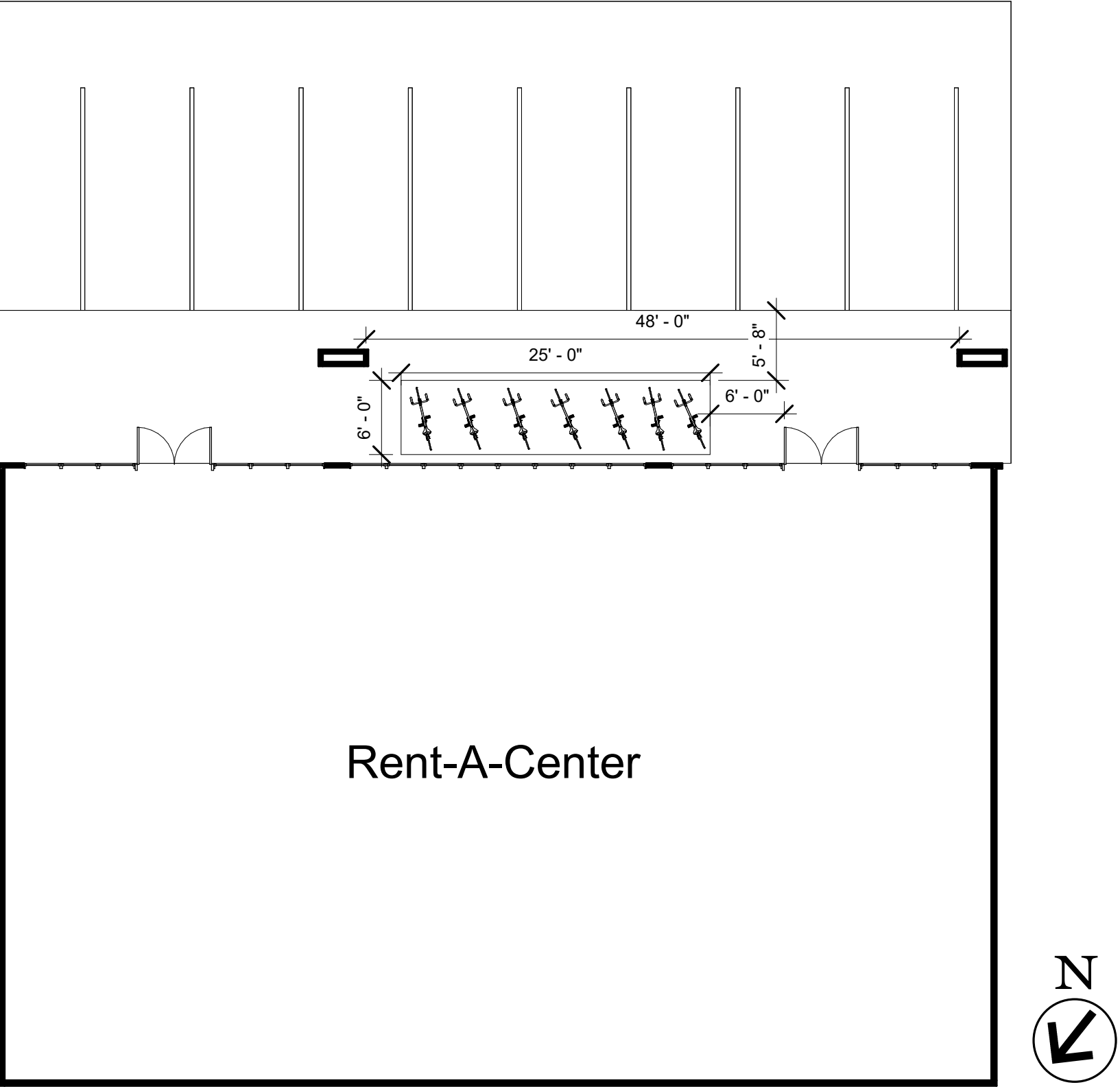
① Level 1 3/32" = 1'-0"
