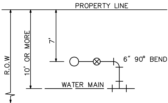
C. WATER MAIN MORE THAN 10' FROM PL HYDRANT LOCATED AT 7' FROM PL (WHEN REQUIRED BY O.C.R.C.)
