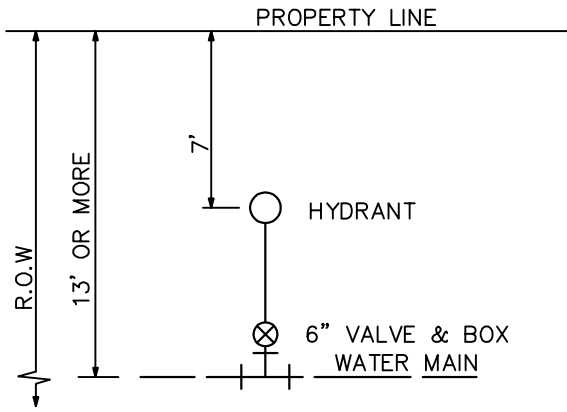
A. WATER MAIN MORE THAN 13' FROM PL HYDRANT LOCATED AT 7' FROM PL (WHEN REQUIRED BY O.C.R.C.)
