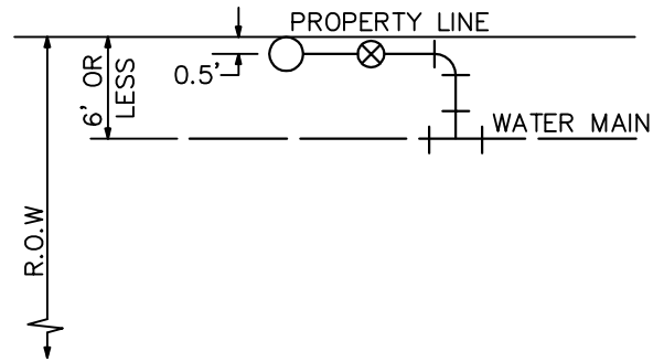
D. WATER MAIN LESS THAN 6' FROM PL HYDRANT LOCATED AT 0.5' FROM PL
