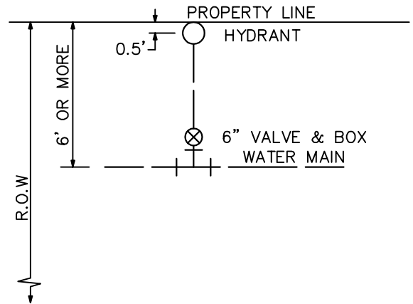
B. WATER MAIN MORE THAN 6' FROM PL HYDRANT LOCATED AT 0.5' FROM PL
